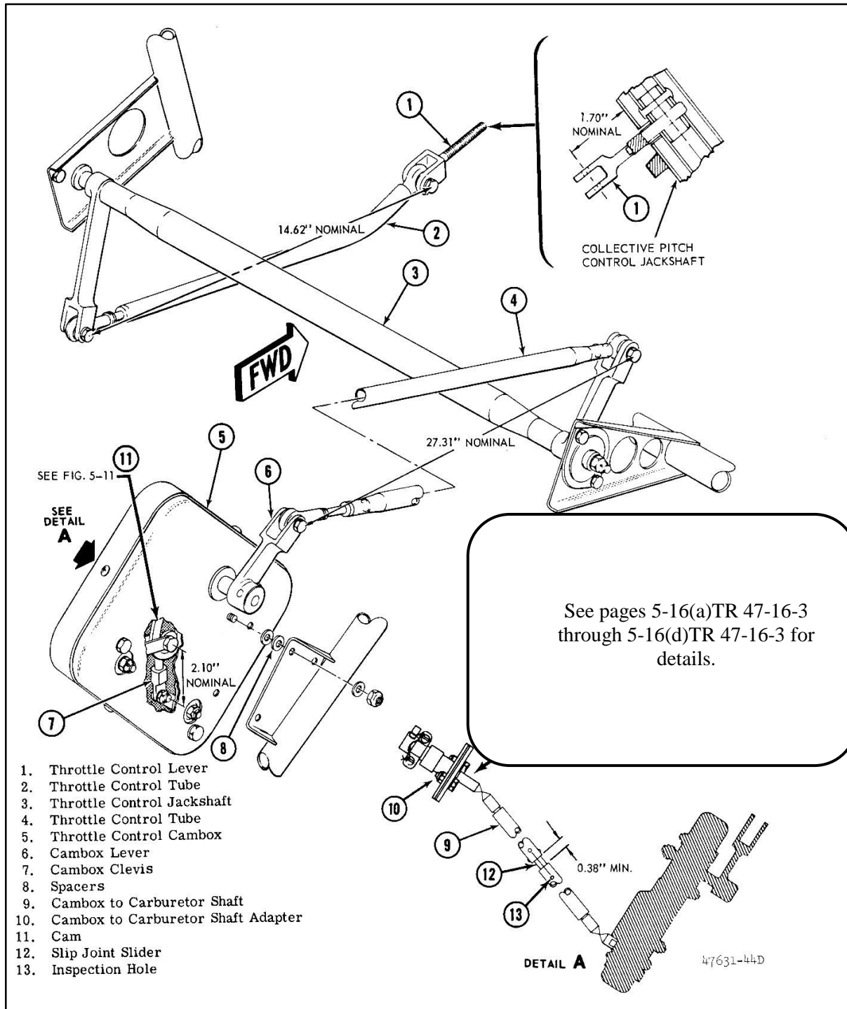
Figure 5-11. Throttle Control Installation
